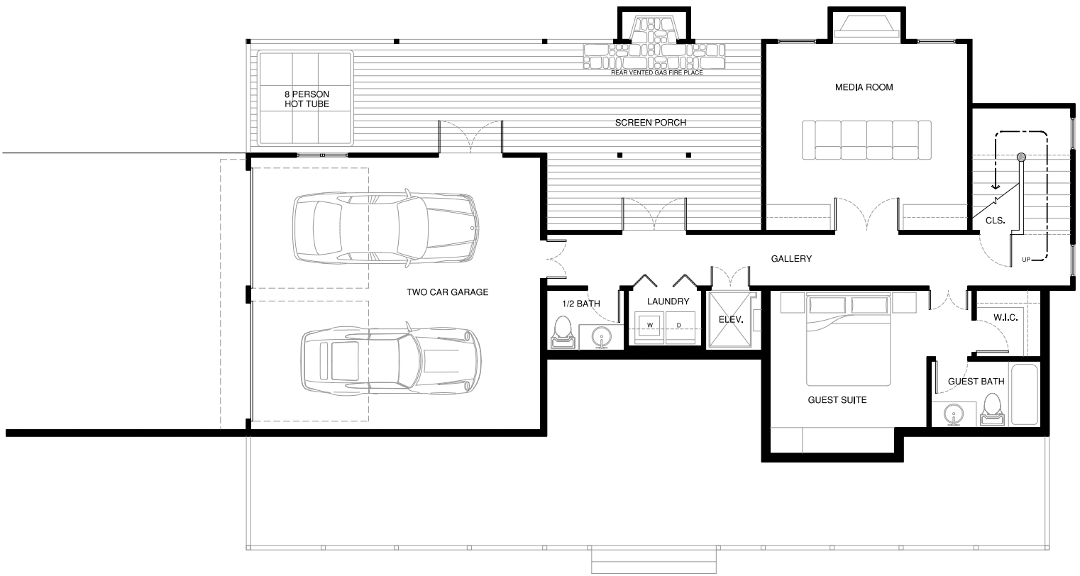
LOWER LEVEL FLOOR PLAN AREA = 809 SF SCALE: 1/4" = 1'-0"
