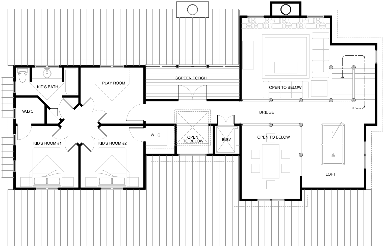
UPPER LEVEL FLOOR PLAN AREA = 869 SF SCALE: 1/4" = 1'-0"
